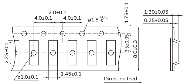
PRG21_RK Series: Embossed Tape
