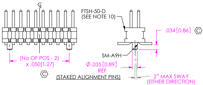
SEE NOTE 12 FIG 2 -K OPTION (LEAD STYLE -01 ONLY) (DIFFERENT AS SHOWN, OTHERWISE SAME AS FIG 1) (POSITION 13, 17, 20 & 25 AVAILABLE WITH -EXX OPTION)
