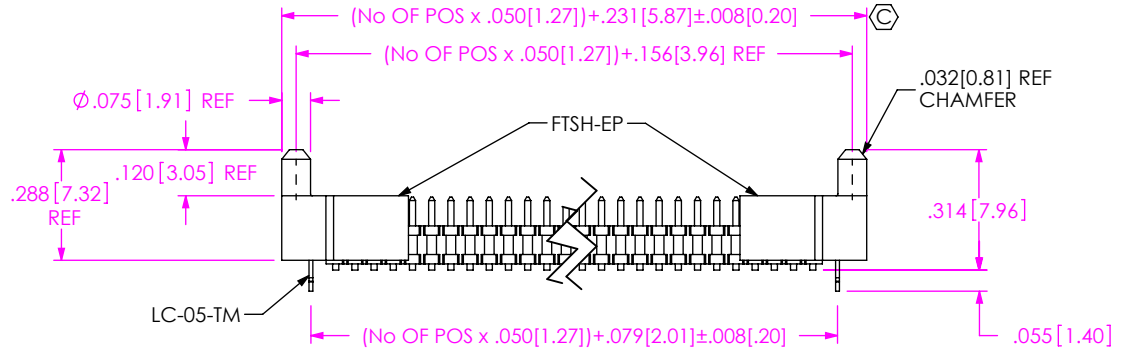
FIG 10 -EPC OPTION (DIFFERENT AS SHOWN, OTHERWISE SAME AS FIG 6) (USE ONLY WHEN MATING WITH CLP)
