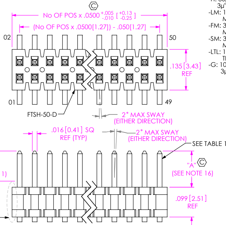
FIG 1 FTSH-1XX-XX-XXX-DV SHOWN
