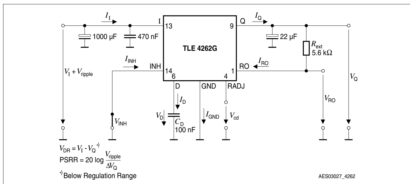
Figure 4 Test circuit
