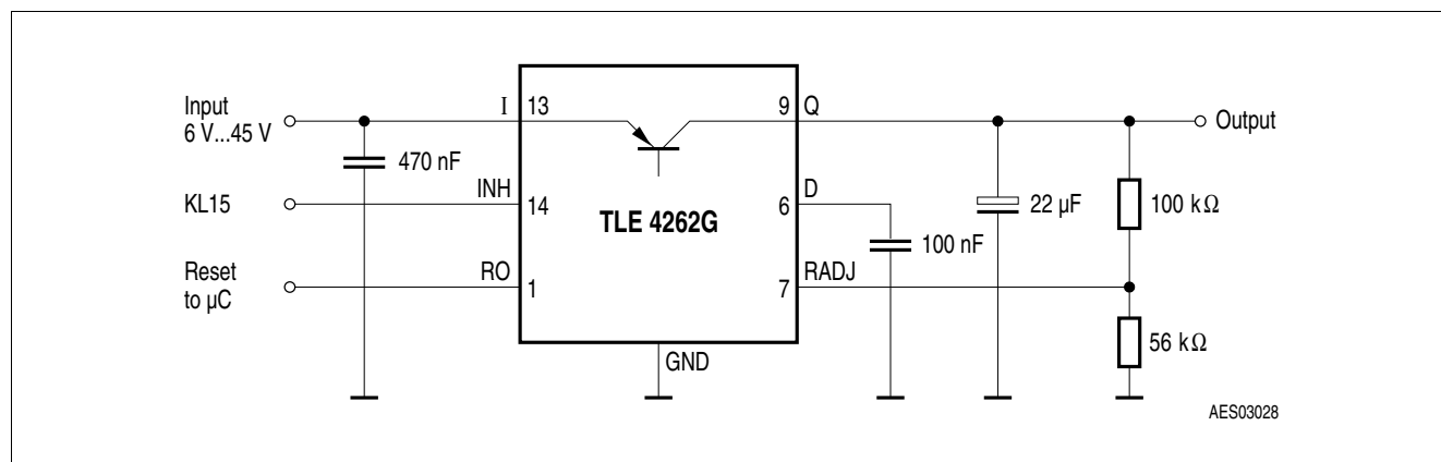
Figure 3 Application circuit
