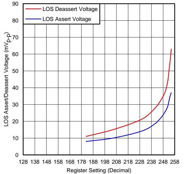
LOS ASSERT / DEASSERT VOLTAGE vs REGISTER SETTING (LOSRNG = 0)
