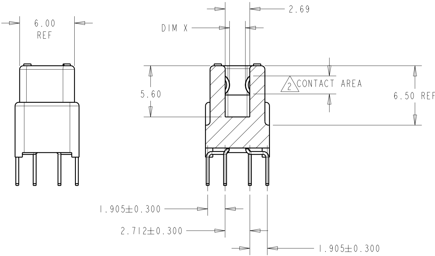
SECTION X-X
