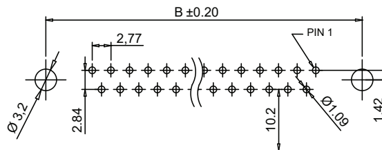
EDGE OF P.C.BOARD RECOMMENDED P.C.B LAYOUT (TOP VIEW) TOLERANCES: \pm 0.05\text{mm}
