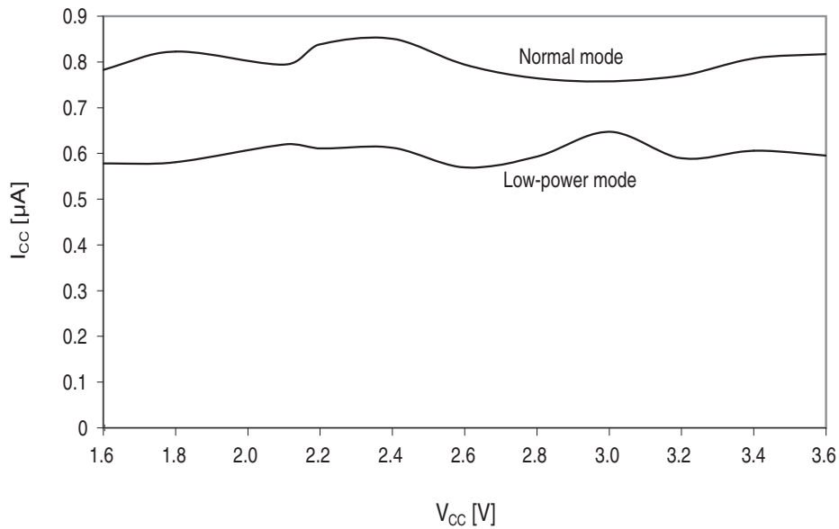
Figure 34-18. Power-save Mode Supply Current vs. V_{CC}
