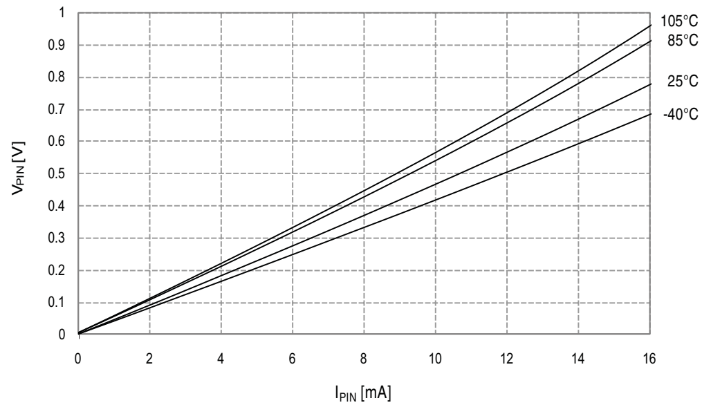
Figure 34-109. I/O Pin Output Voltage vs. Sink Current
