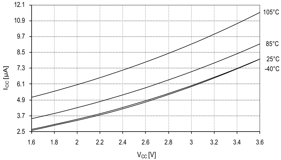
Figure 34-98. Standby Supply Current vs. V_{CC} Standby, f_{SYS} = 1MHz
