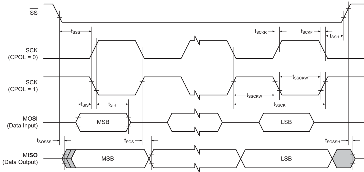
Figure 33-13. SPI Timing Requirements in Slave Mode
