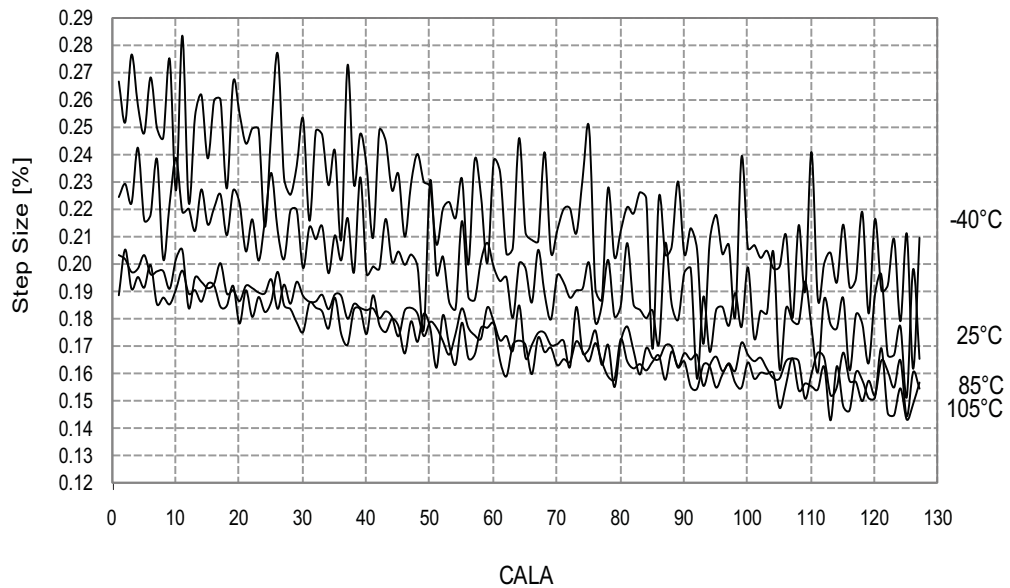
Figure 34-70. 2MHz Internal Oscillator CALA Calibration Step Size
