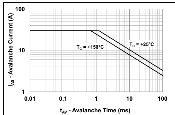
FIGURE 2-12: Single-Pulse Unclamped Inductive Switching.
