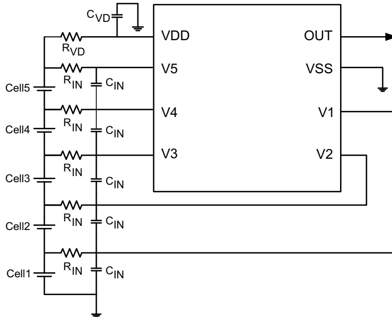
Figure 9-1. Application Configuration
