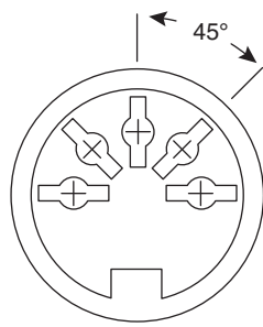
5 Contacts 161-0005-E
