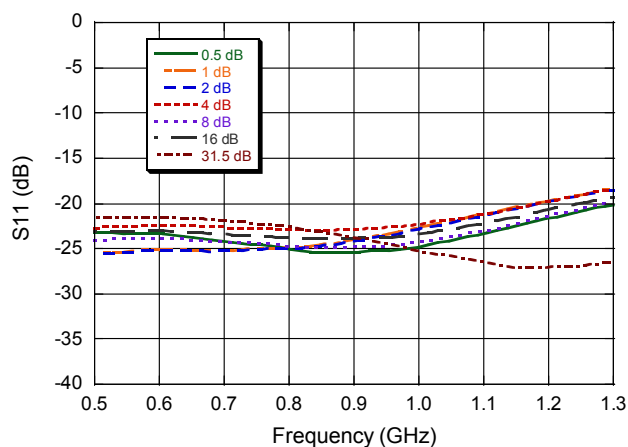
Input Return Loss, across all attenuation states
