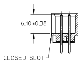
SECTION E-E
