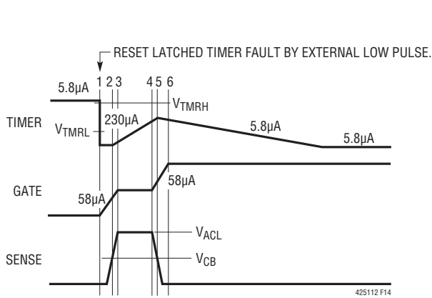
Figure 14. Latched Fault Reset Timing (All Waveforms are Referenced to V_{EE} )
