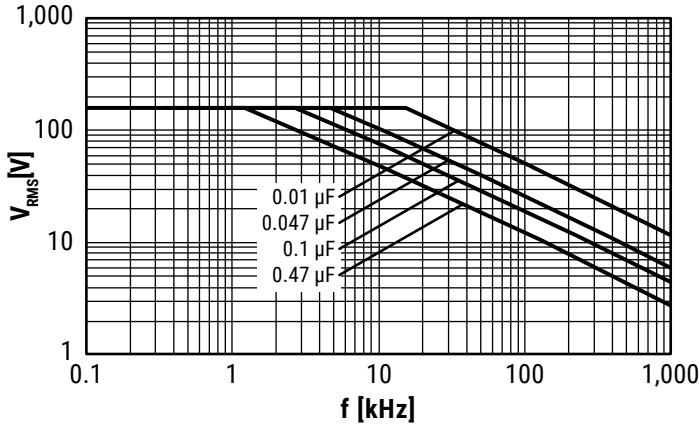
400 VDC/160 VAC
