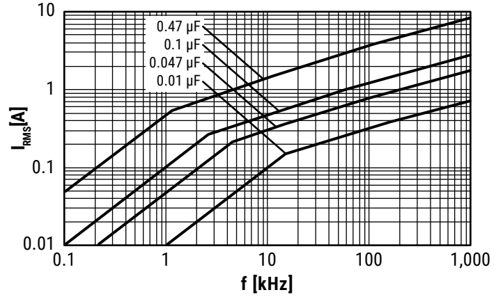
400 VDC/160 VAC
