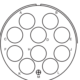
Insert Arrangement 40-72 Service Rating A Number of Contacts 1 10 Contact Size 16 4 (Coax) RG-9B/U
