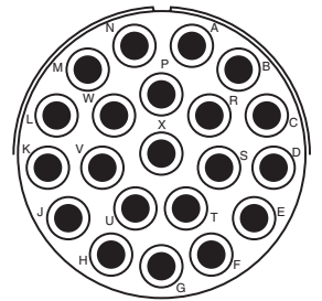
Insert Arrangement 40-68 Service Rating A Number of Contacts 21 Contact Size 8
