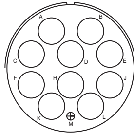
Insert Arrangement 40-67 Service Rating A Number of Contacts 1 10 Contact Size 16 4 (Coax) RG-59/U
