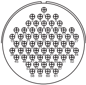
Insert Arrangement 40-70 Service Rating A Number of Contacts 61 Contact Size 16
