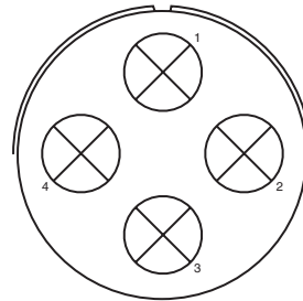
Insert Arrangement 40-66 Service Rating - Number of Contacts 4 Contact Size 0 (Coax) RG-63B/U
