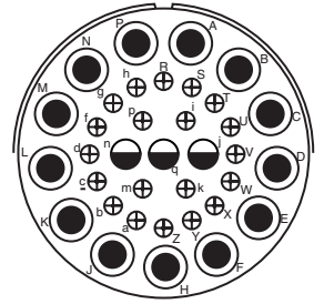
Insert Arrangement 40-64 Service Rating - Number of Contacts 3 20 13 Contact Size 12 16 8 (Coax) RG-124/U
