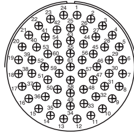
Insert Arrangement 40-63 Service Rating A Number of Contacts 61 Contact Size 16 for #14 wire
