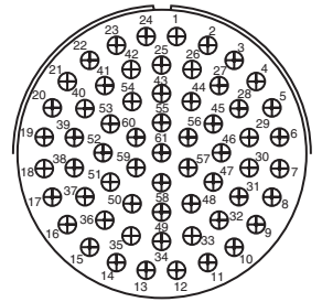
Insert Arrangement 40-73 Service Rating A Number of Contacts 61 Contact Size 16
