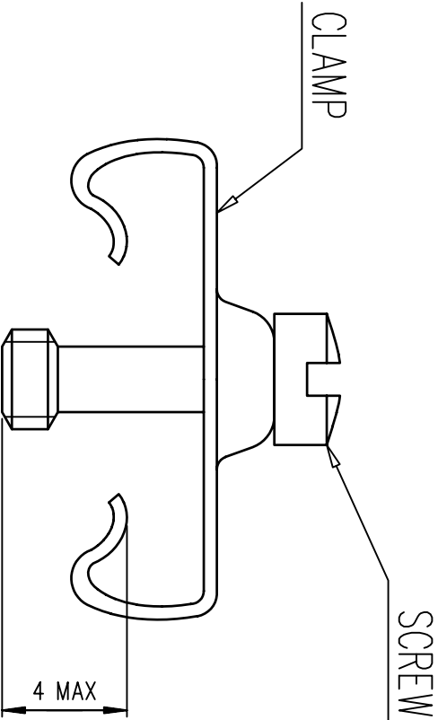
VIEW ASSEMBLY
