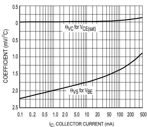
Figure 15. Temperature Coefficients
