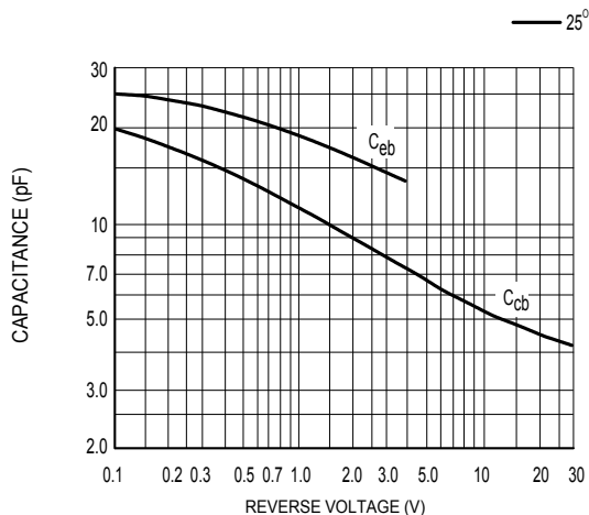
Figure 1. Capacitances
