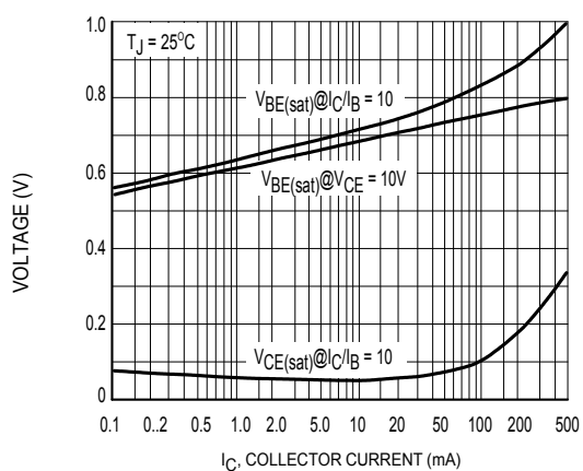
Figure 14. "ON" Voltages
