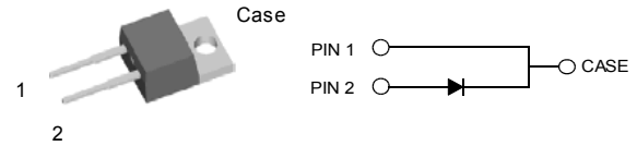
TO – 220AC
