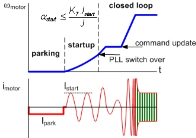
Figure 7 Starting sequence
