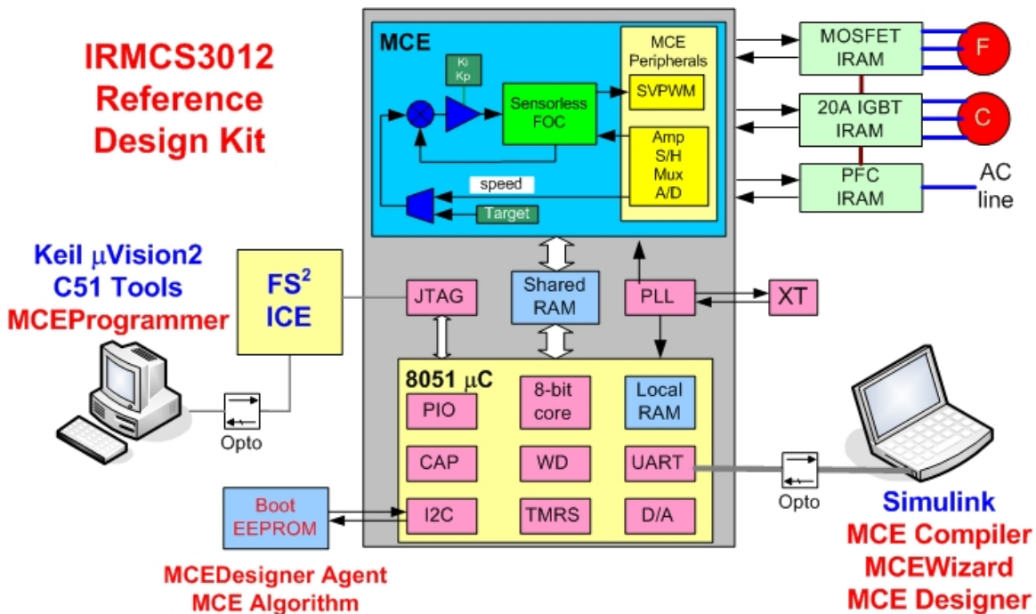
Figure 11 IRMCx300 Reference Design Kit
