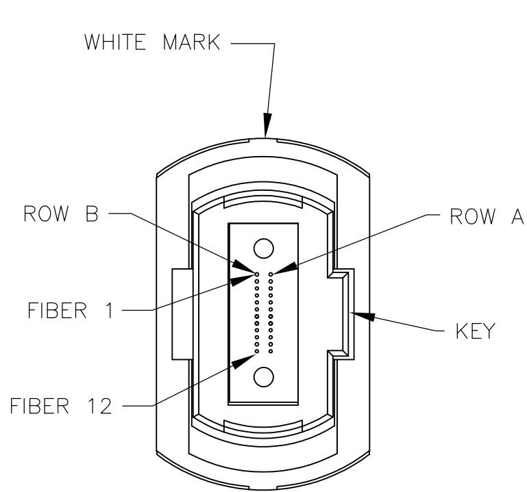
VIEW Z-Z NOT TO SCALE
