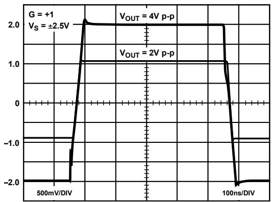
Figure 33. Large Signal Transient Response, G = +1
