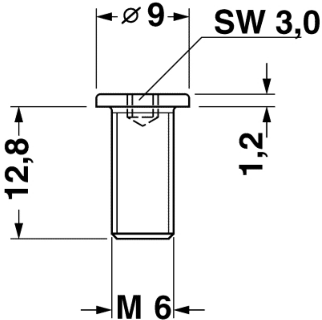
Dimensional drawing
