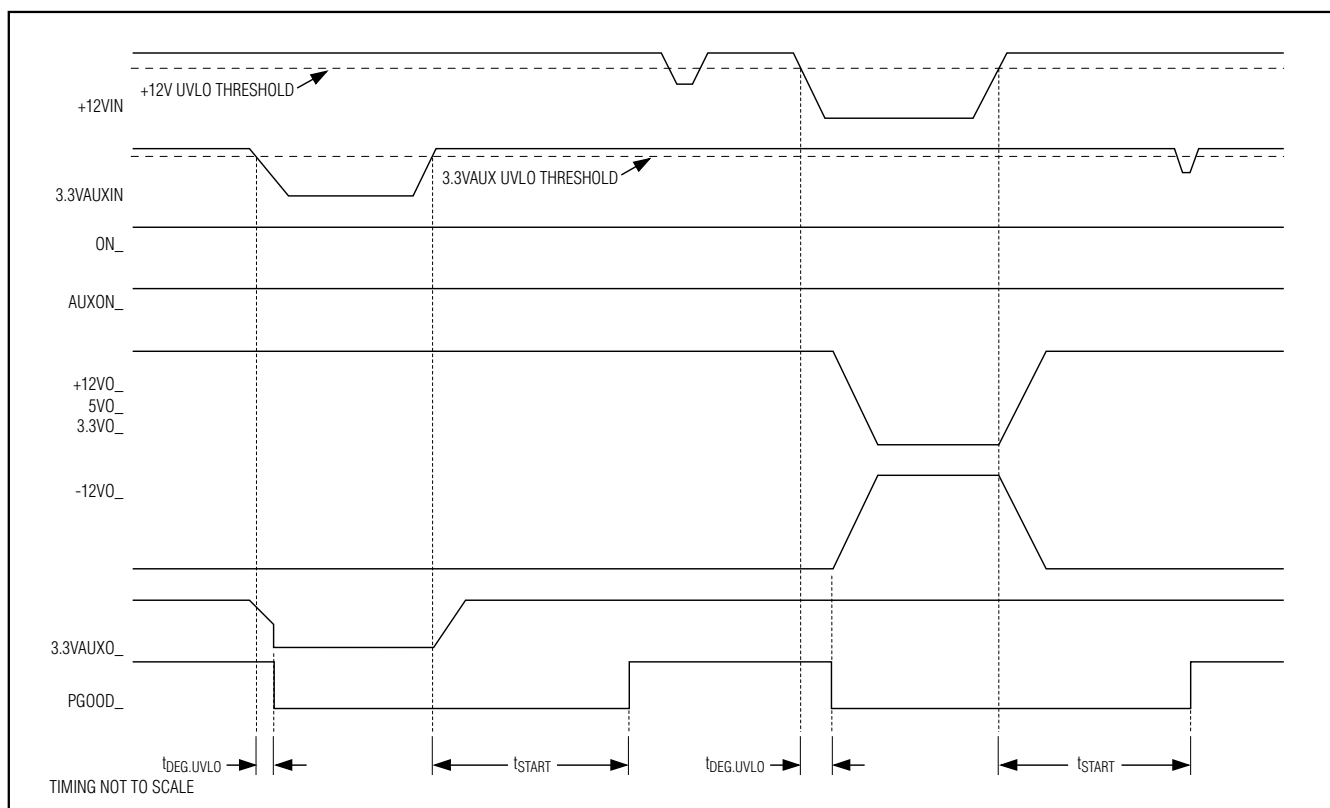
Figure 2. Input UVLO Fault Management in the MAX5915/MAX5915A/MAX5916/MAX5916A
