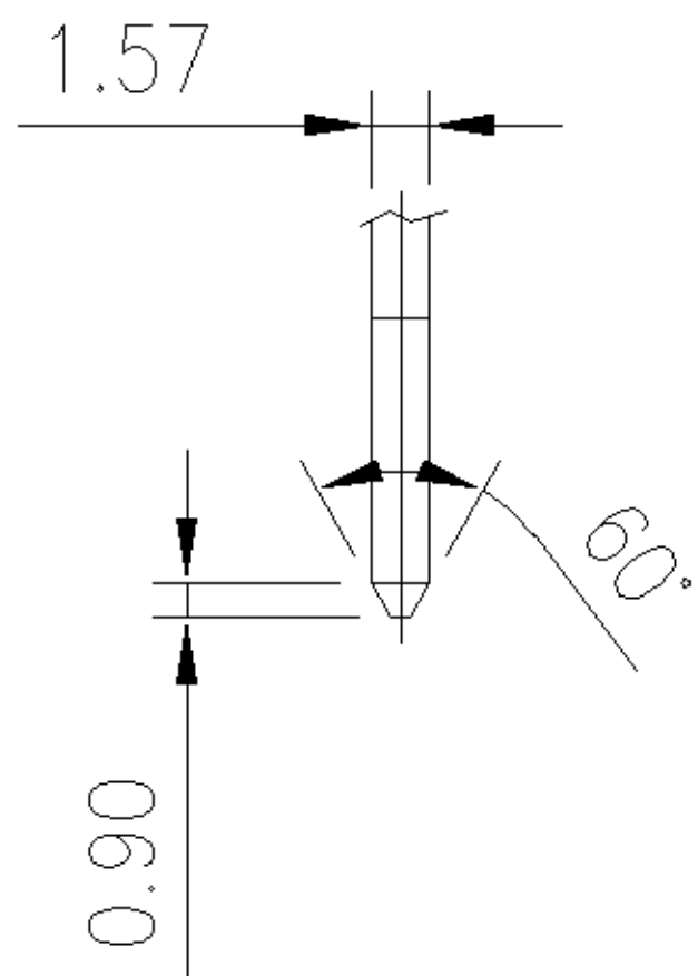
TYPICAL CARD EDGE PROFILE
