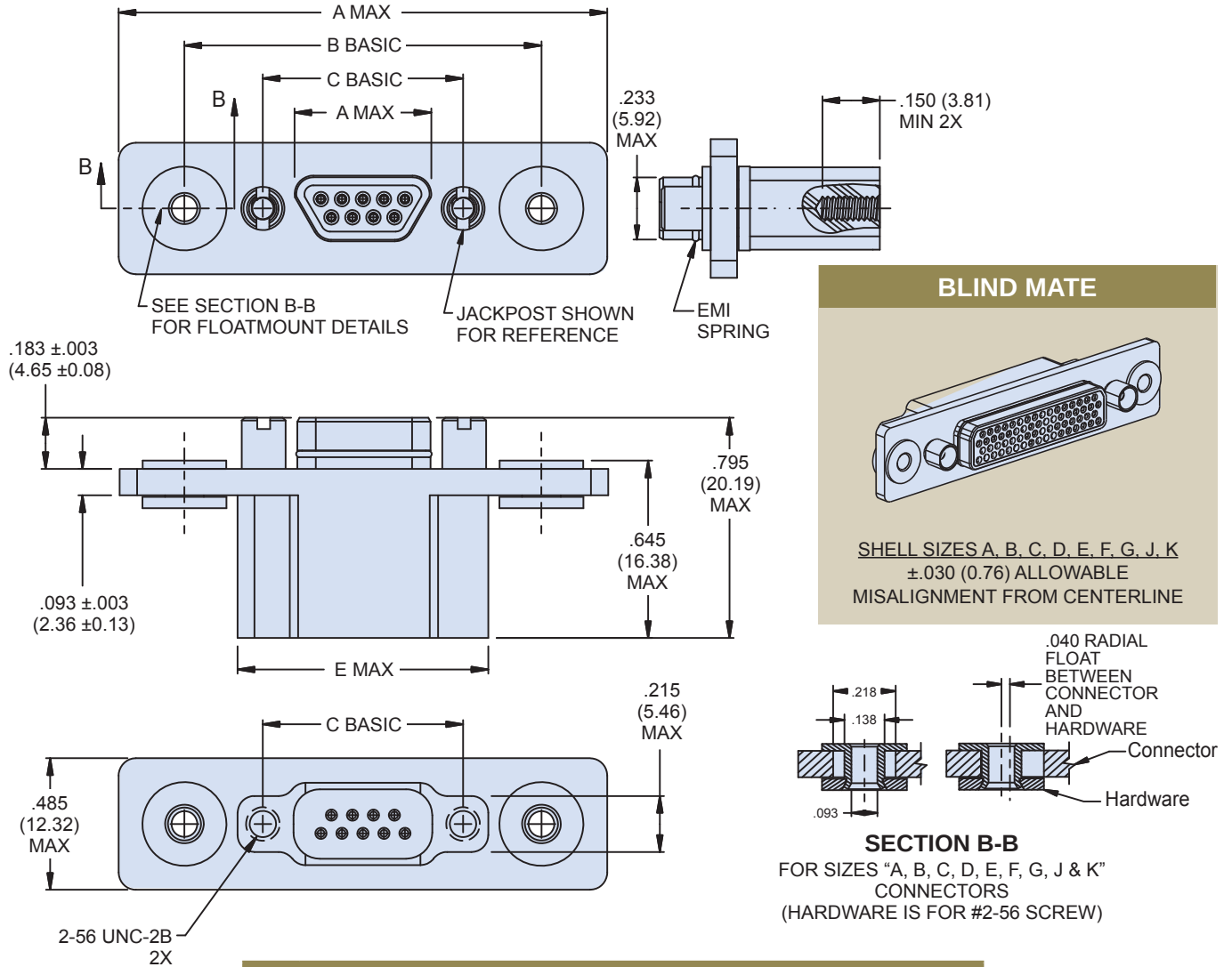
790-049S SIZES A, B, C, D, E, F, G, J & K DIMENSIONS
