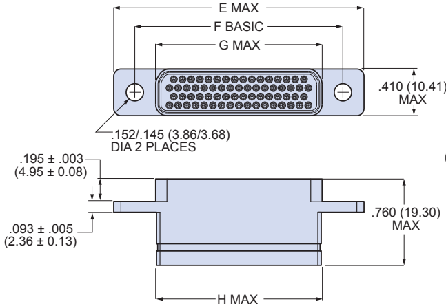
SHELL SIZE H AND L
