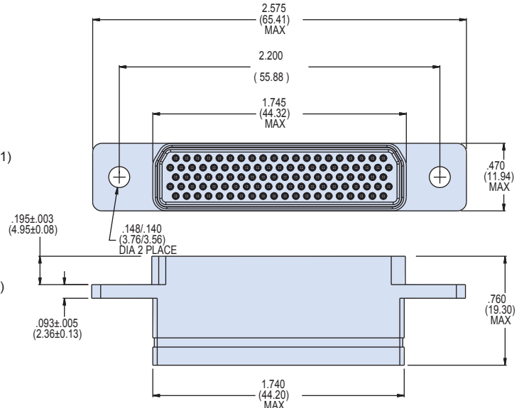
SHELL SIZE M
