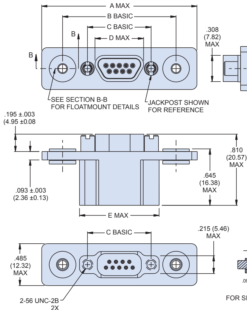
790-050P SIZES A, B, C, D, E, F, G, J & K DIMENSIONS
