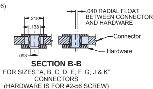
790-050P SIZES A, B, C, D, E, F, G, J & K DIMENSIONS
