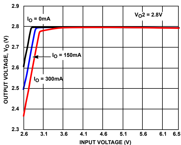
FIGURE 5. OUTPUT VOLTAGE vs INPUT VOLTAGE ( V_{O2} = 2.8\text{V} )
