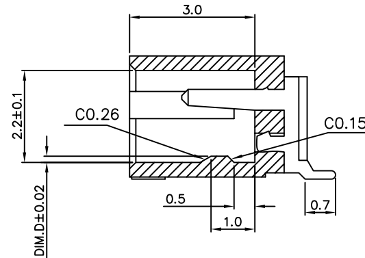
SECTION X-X
