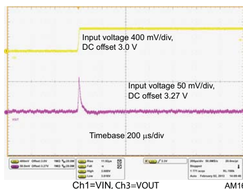
Figure 11. Line transient response @ V_{IN} = 3\text{ V} to 3.6\text{ V}
