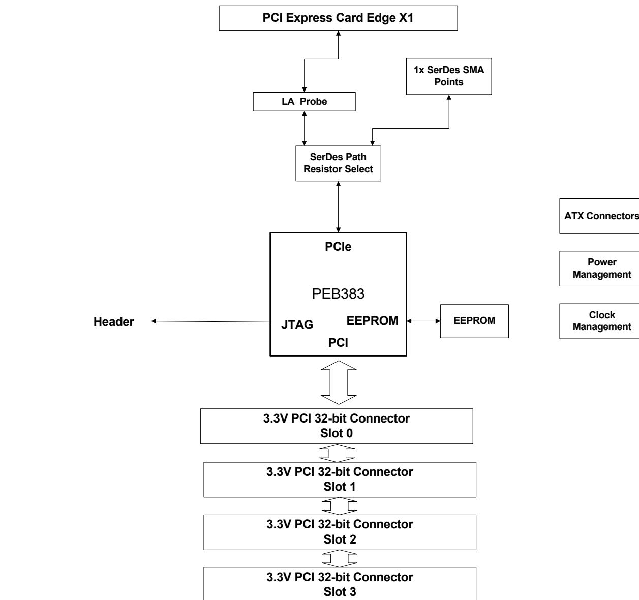
Figure 1: Evaluation Board Block Diagram
