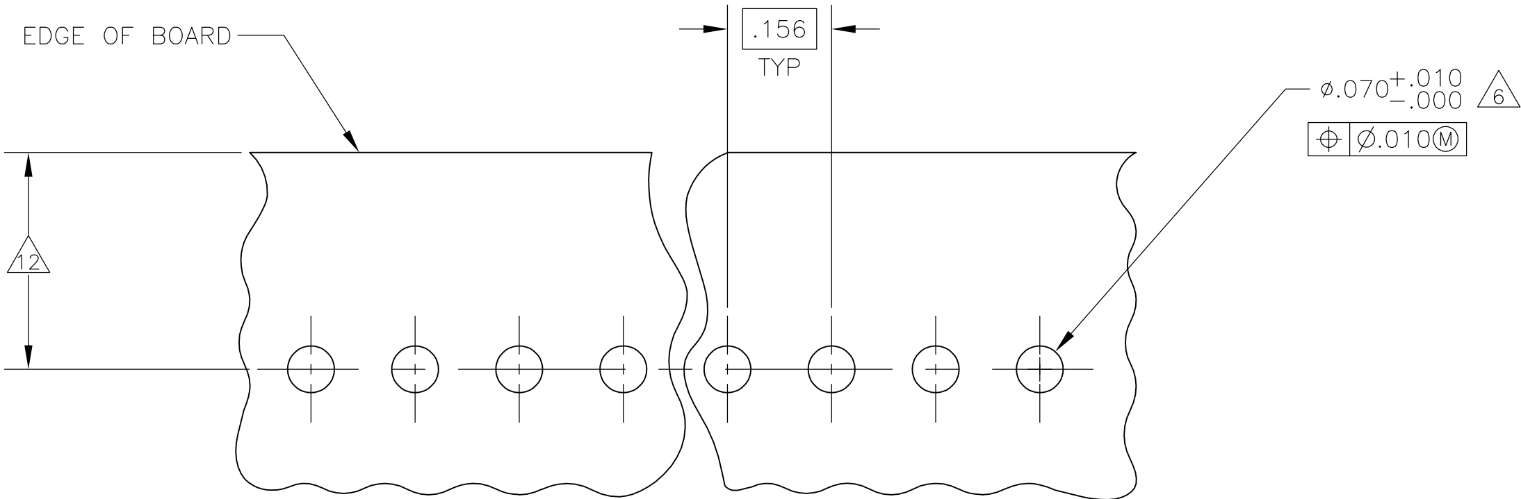
RECOMMENDED MOUNTING HOLE PATTERN FOR .109±0.016 THICK P.C. BOARD
