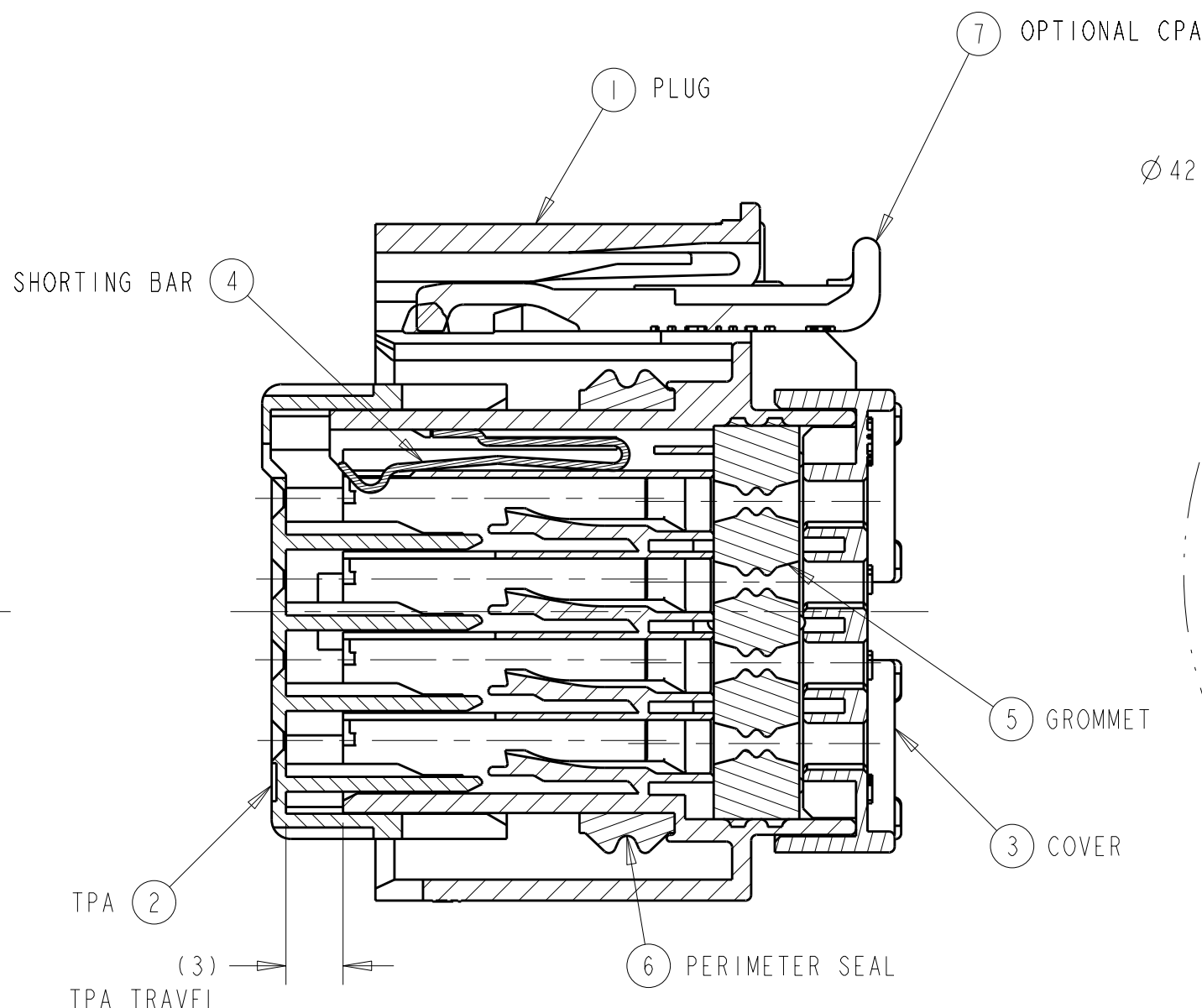
SECTION A-A SHOWN WITH TPA IN IT'S PRE-LOADED POSITION (DELIVERY CONDNTION)
