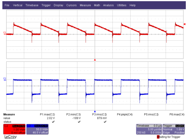
Figure 57 – 132 VAC, 60 Hz. Upper: I D5 , 0.2 A / div. Lower: V D5 , 50 V / div., 5 μs / div.
