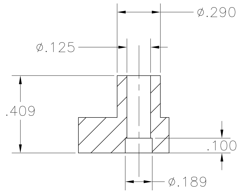
DETAIL A BOTH ENDS
