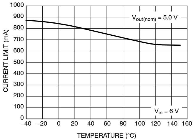
Figure 7. Current Limit vs. Temperature
