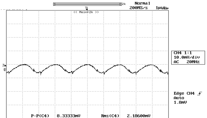
Figure 10: Output ripple & noise at 12Vin, 2.5V/20A out
