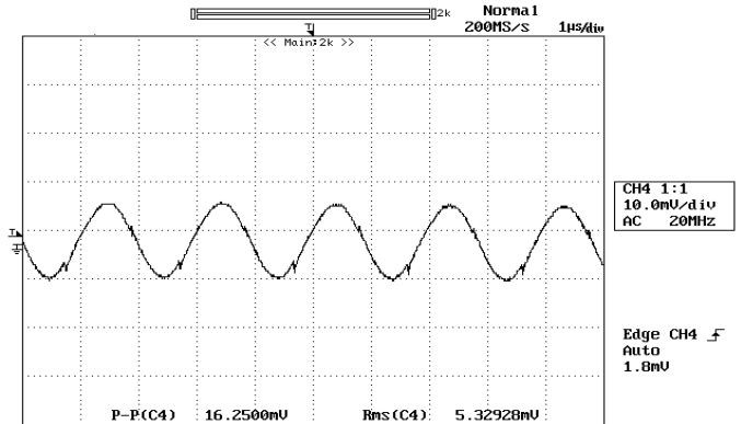
Figure 12: Output ripple & noise at 12Vin, 5.0V/20A out
