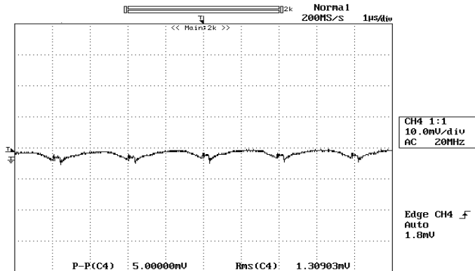
Figure 8: Output ripple & noise at 12Vin, 0.9V/20A out
