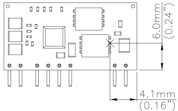
Figure 25: Temperature measurement location* The allowed maximum hot spot temperature is defined at 130 °C
