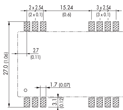
Pin Patterns:
