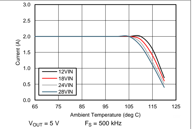
Figure 62. Derating Curve
