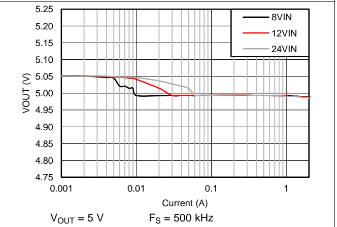
Figure 60. Regulation Curve
