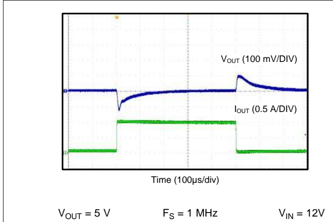
Figure 61. Load Transient 0.1A to 1A
