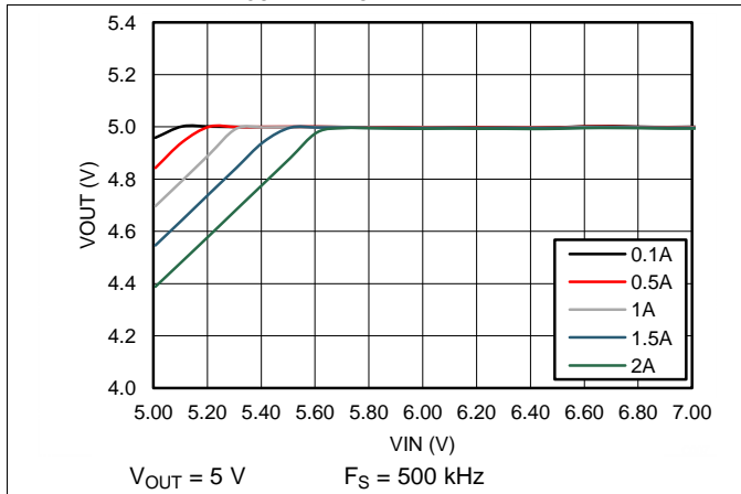
Figure 57. Dropout Voltage
