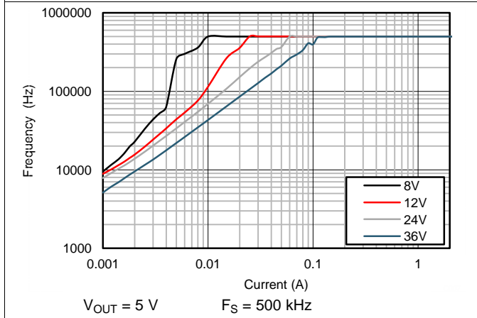
Figure 59. Frequency vs Load
