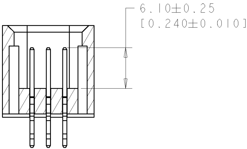
SECTION Z-Z
