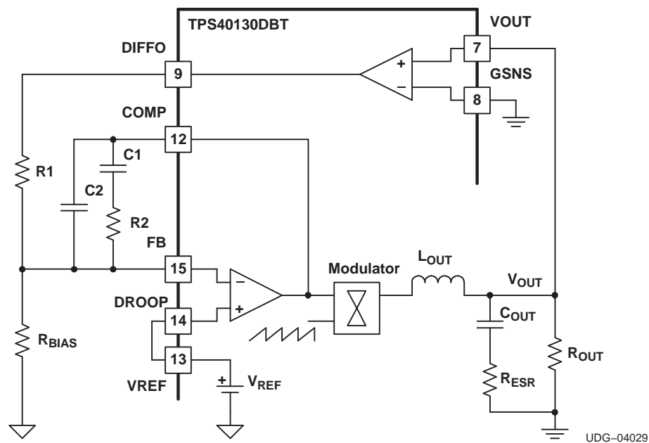
Figure 5. Compensation Components
