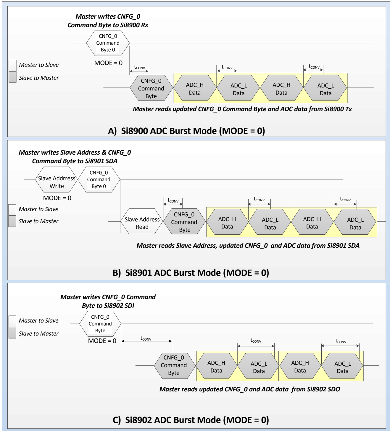
Figure 5. ADC Burst Mode Operation
