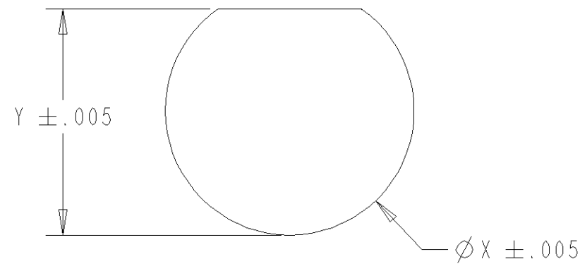
RECOMMENDED PANEL CUTOUT DIMENSIONS
