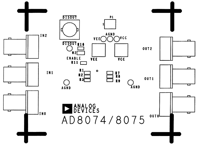
Figure 8. Silkscreen Top
