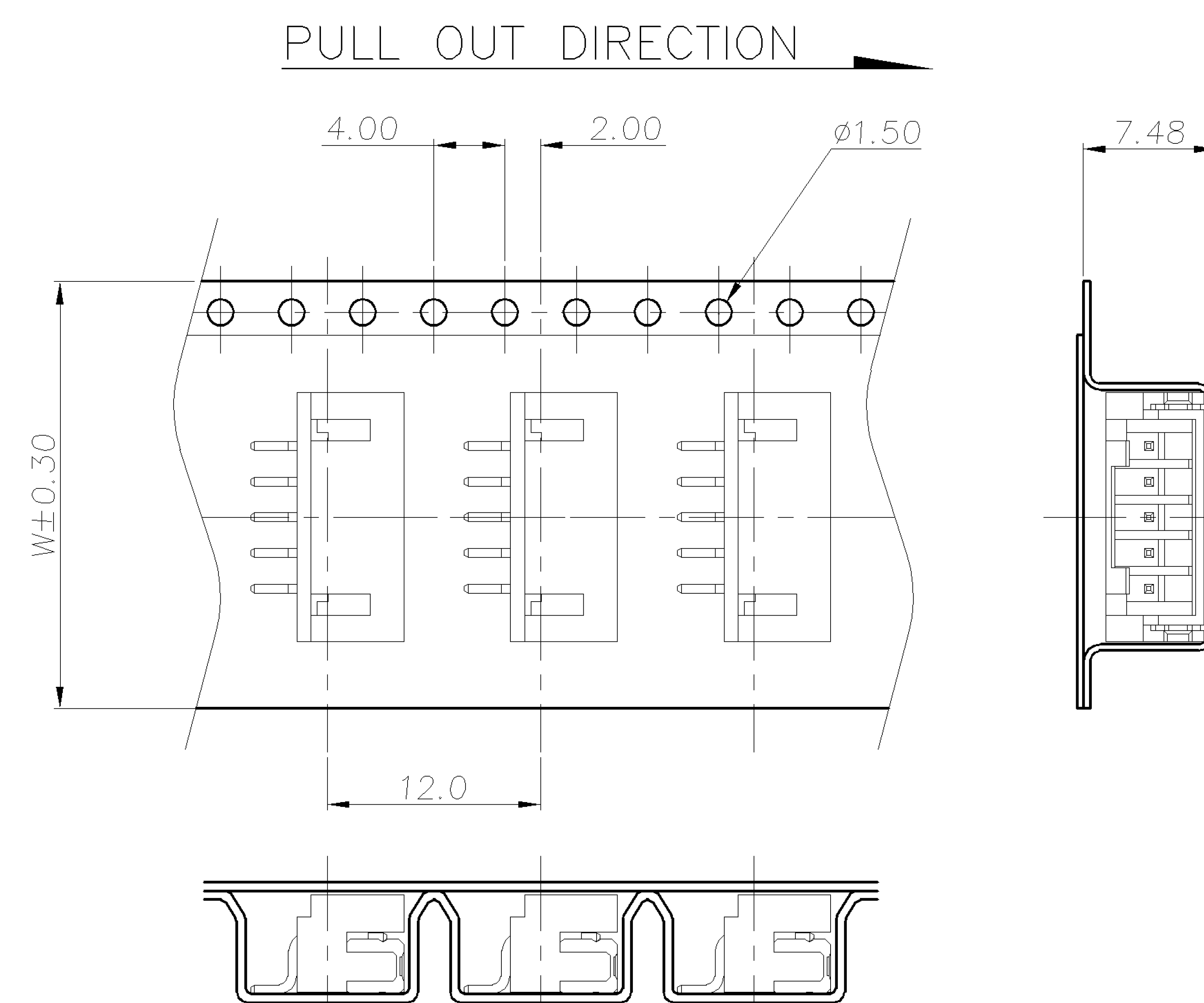
PRODUCT LOADING FOR 2 TO 6 CONTACTS
