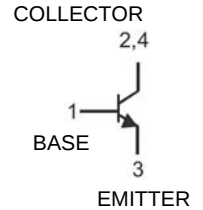
Schematic and Pin Configuration
