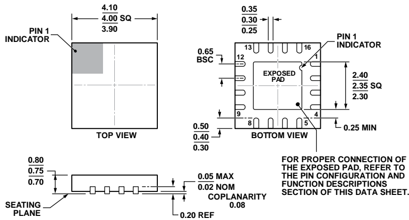
COMPLIANT TO JEDEC STANDARDS MO-220-WGGC-3. Figure 57. 16-Lead Lead Frame Chip Scale Package [LFCSP_WQ] 4 mm x 4 mm Body, Very Very Thin Quad (CP-16-20) Dimensions shown in millimeters
