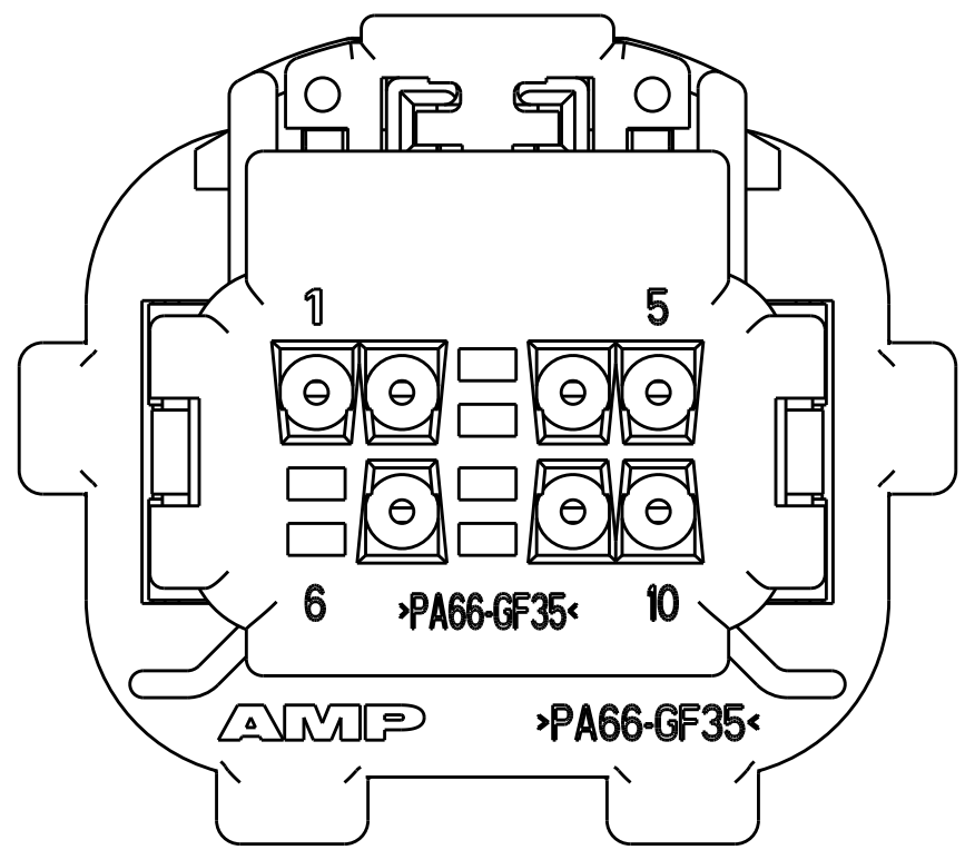
VIEW SHOWS COVER, FOR 2-638517-1
