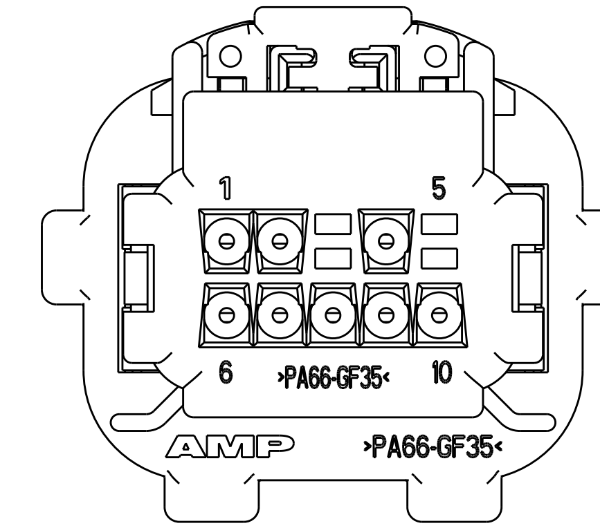
VIEW SHOWS COVER, FOR 2-638517-9
