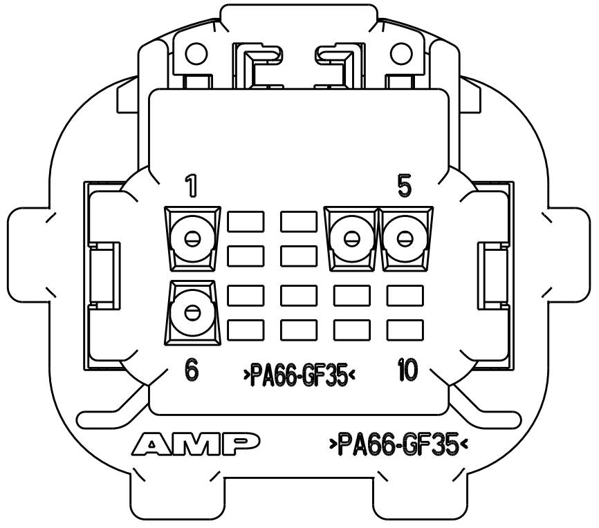
VIEW SHOWS COVER, FOR 2-638517-6
