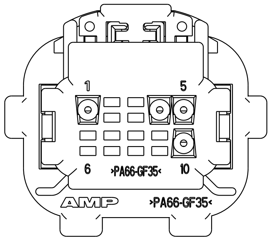
VIEW SHOWS COVER, FOR 2-638517-3
