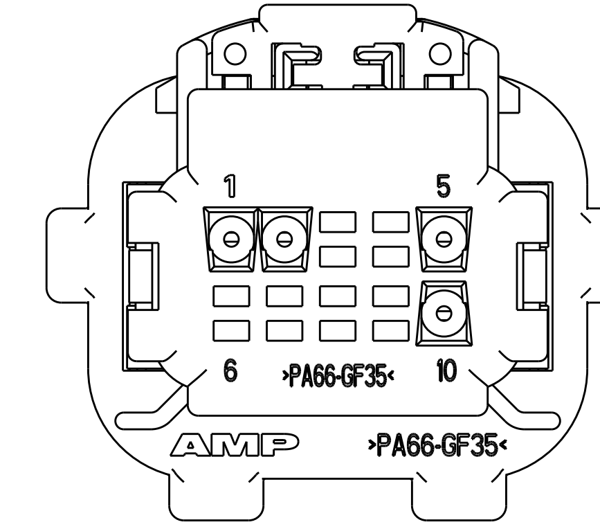
VIEW SHOWS COVER, FOR 2-638517-7
