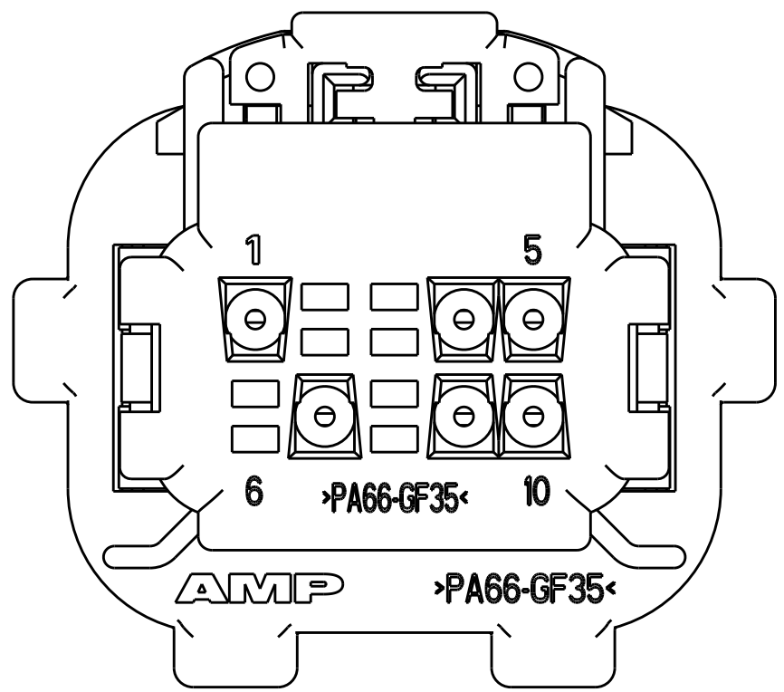
VIEW SHOWS COVER, FOR 2-638517-2
