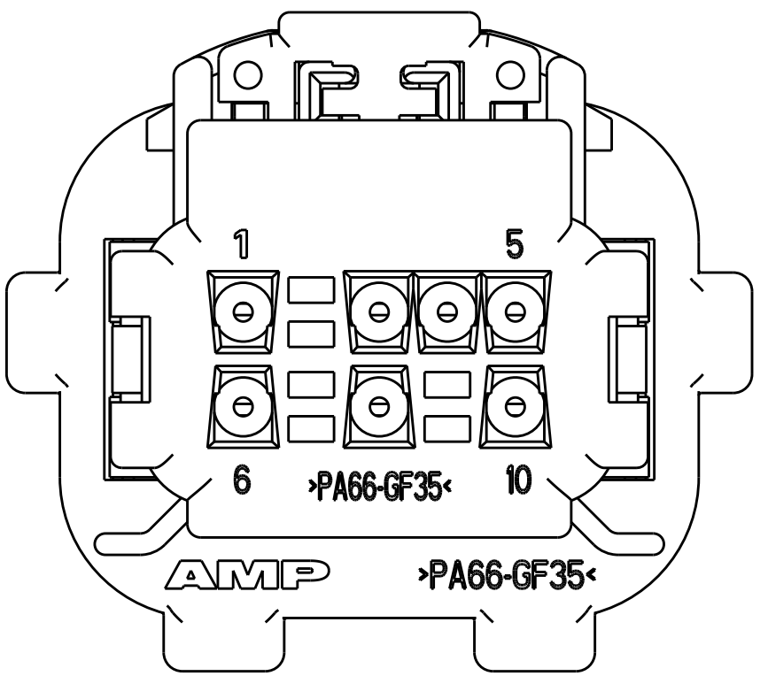
VIEW SHOWS COVER, FOR 2-638517-4 & 5-638517-4
