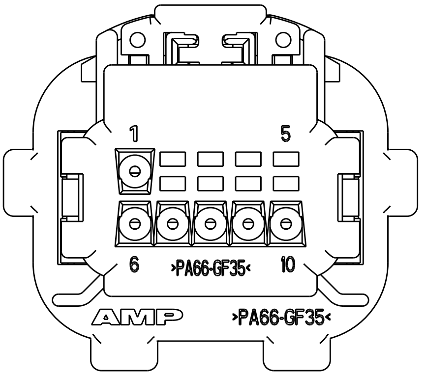
VIEW SHOWS COVER, FOR 3-638517-0
