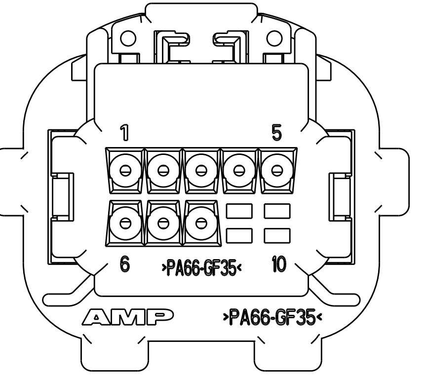
VIEW SHOWS COVER, FOR 2-638517-8
