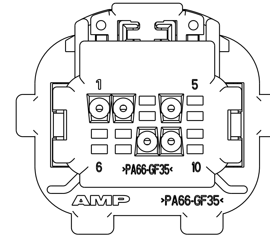
VIEW SHOWS COVER, FOR 3-638517-1
