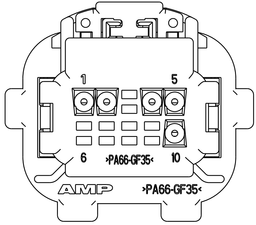
VIEW SHOWS COVER, FOR 2-638517-5
