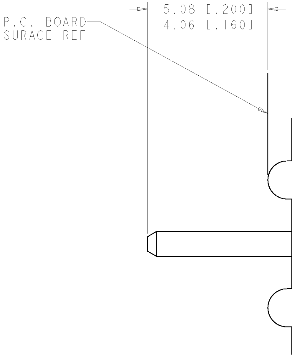
8. SOLDER PIN DETAIL SCALE 10 : 1
