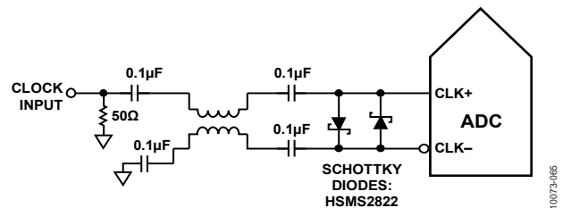
Figure 62. Balun-Coupled Differential Clock (Up to 1 GHz)
