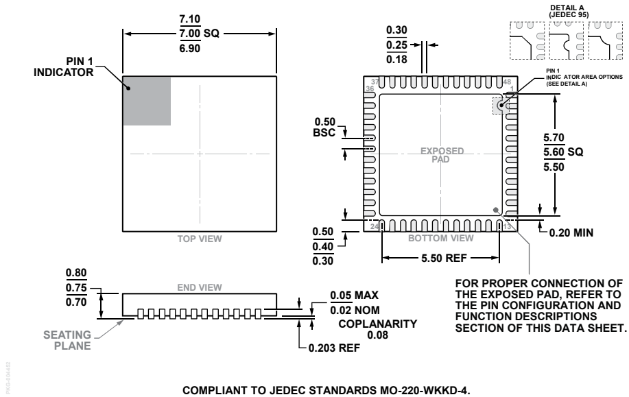
Figure 76. 48-Lead Lead Frame Chip Scale Package [LFCSP] 7 mm × 7 mm Body and 0.75 mm Package Height (CP-48-13) Dimensions shown in millimeters
