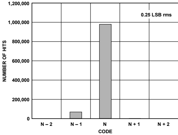
Figure 42. Input-Referred Noise Histogram, f_{SAMPLE} = 125 MSPS
