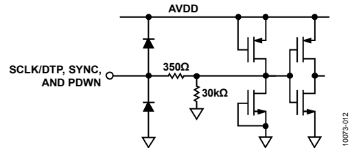
Figure 50. Equivalent SCLK/DTP, SYNC, and PDWN Input Circuit
