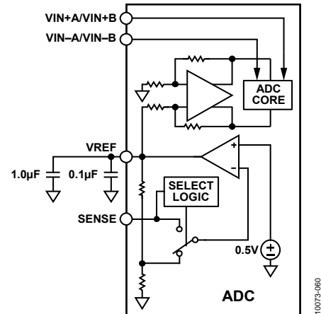
Figure 56. Internal Reference Configuration
