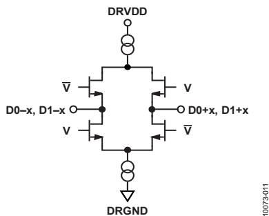
Figure 49. Equivalent Digital Output Circuit
