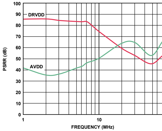
Figure 43. PSRR vs. Frequency, f_{CLK} = 125 MHz, f_{SAMPLE} = 125 MSPS
