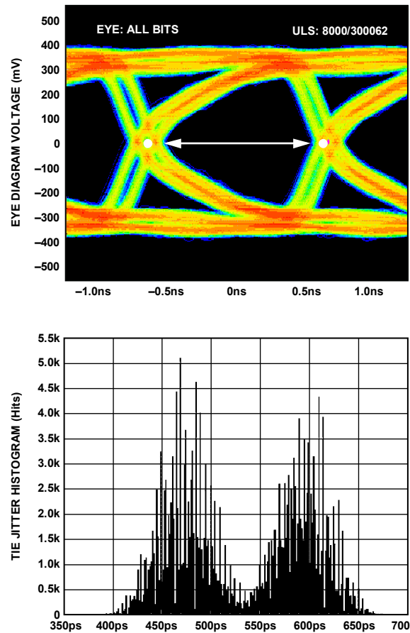
Figure 71. Data Eye for LVDS Outputs in ANSI-644 Mode with Trace Lengths Less than 24 Inches on Standard FR-4 Material, External 100 Ω Far-End Termination Only
