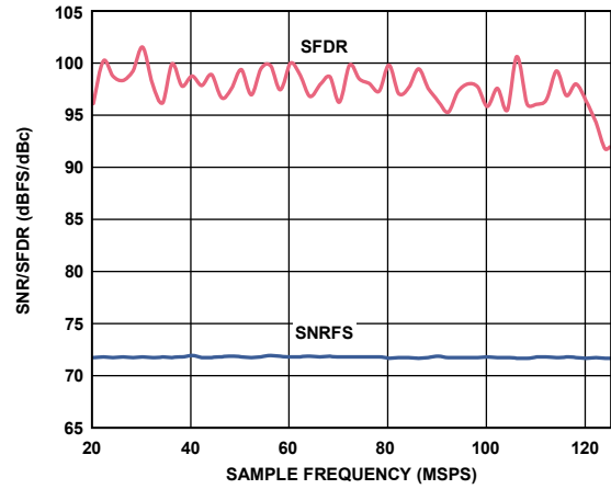
Figure 44. SNR/SFDR vs. Encode, f_{IN} = 9.7 MHz, f_{SAMPLE} = 125 MSPS
