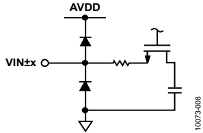
Figure 46. Equivalent Analog Input Circuit
