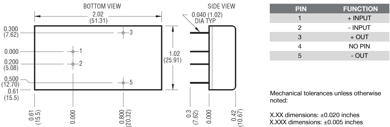
Figure 2. Mechanical Dimensions
