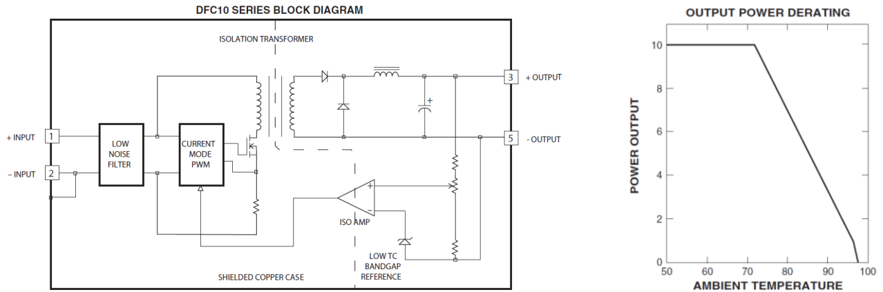
Figure 1. Typical Performance: (Tc = 25°C, Vin = Nom VDC, Rated Load)
