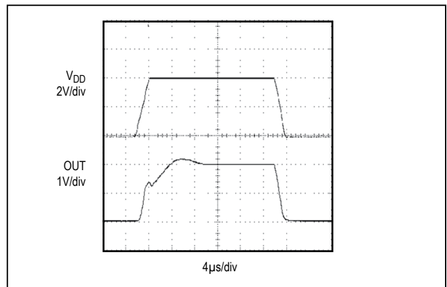
Figure 5. Power-Up/Down Waveform
