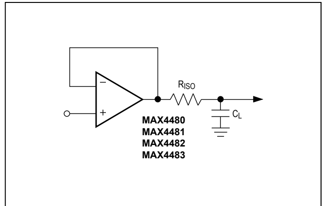
Figure 3. Capacitive-Load-Driving Circuit
