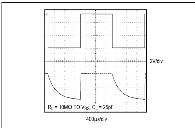
Figure 4. Shutdown Waveform
